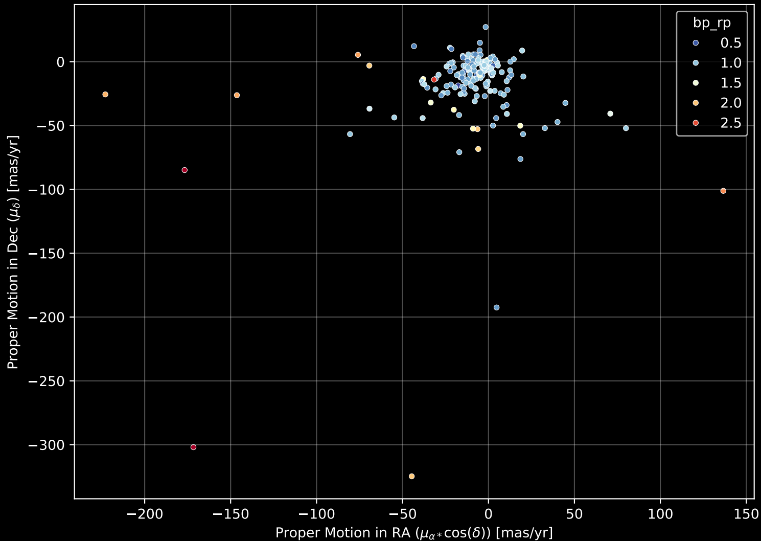
APOGEE DR17 Field: [202+33_MGA] Proper Motion Diagram (n= 181)
