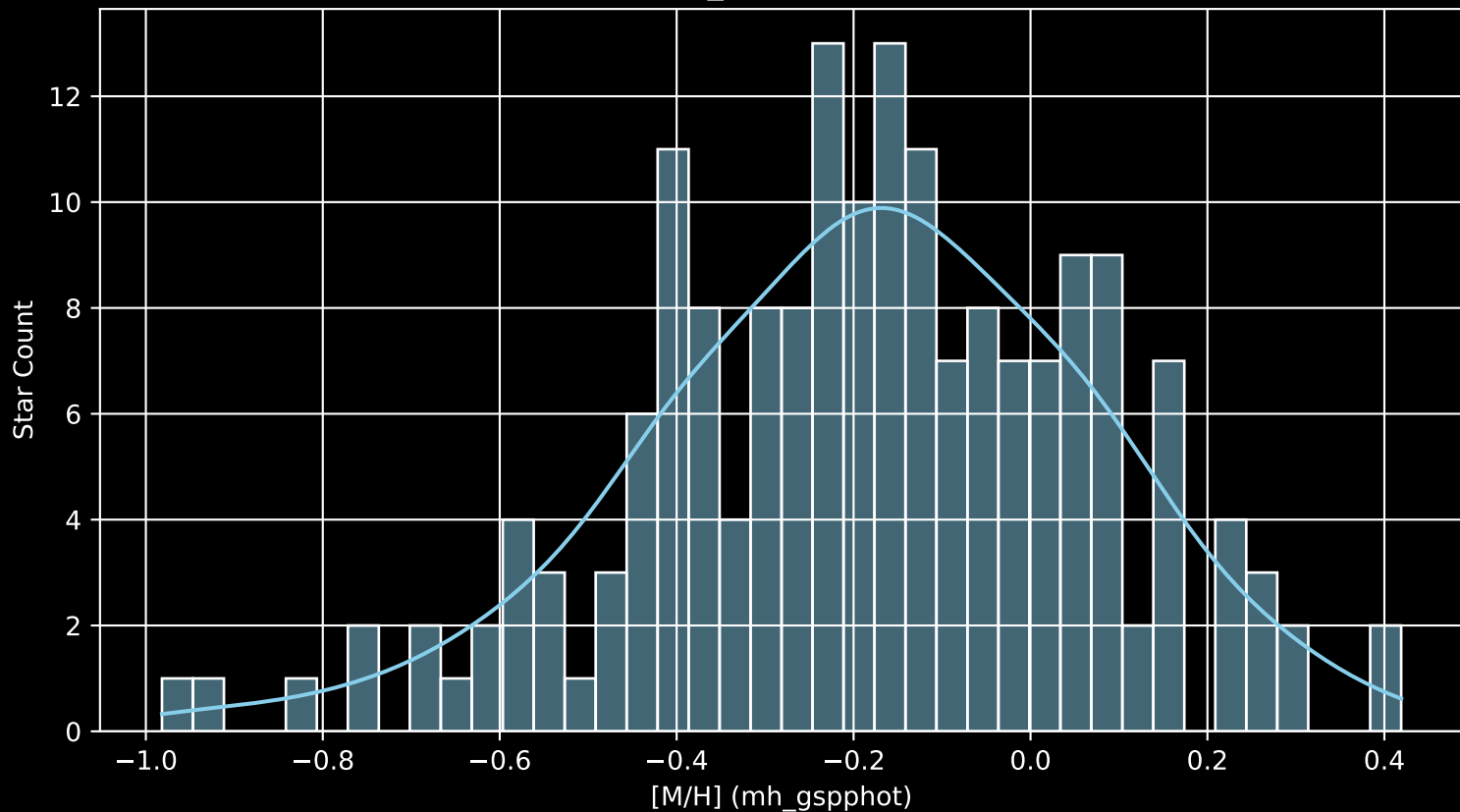
APOGEE DR17 Field: [202+33_MGA [M/H] (mh_gspphot) (n= 180)
