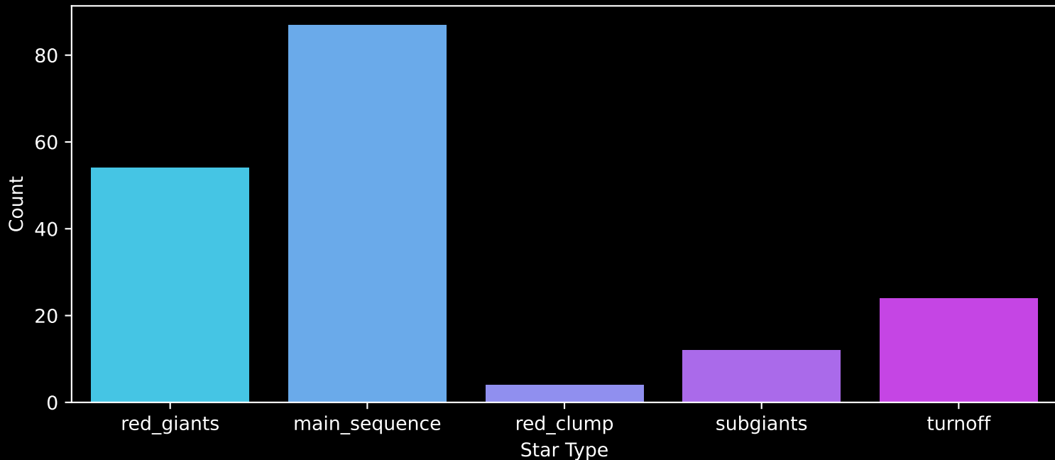
APOGEE DR17 Field: [202+33_MGA] Count plot of Star Type
