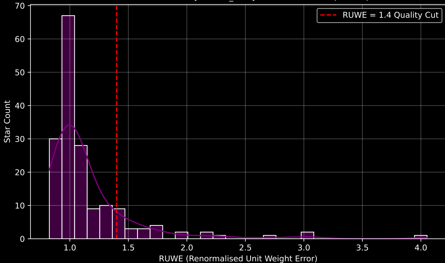
GAPOGEE DR17 Field [202+33_MGA] RUWE Distribution (n= 172)
