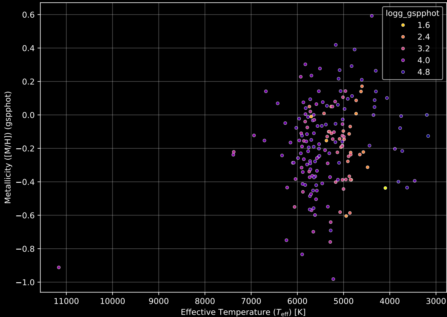
APOGEE DR17 Field: [202+33_MGA] Stellar Population Parameters (n= 181)
