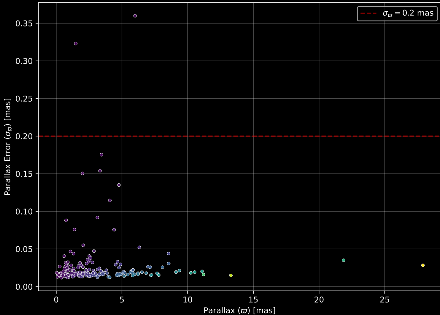
APOGEE DR17 Field: [202+33_MGA] Parallax Quality (n= 181)
